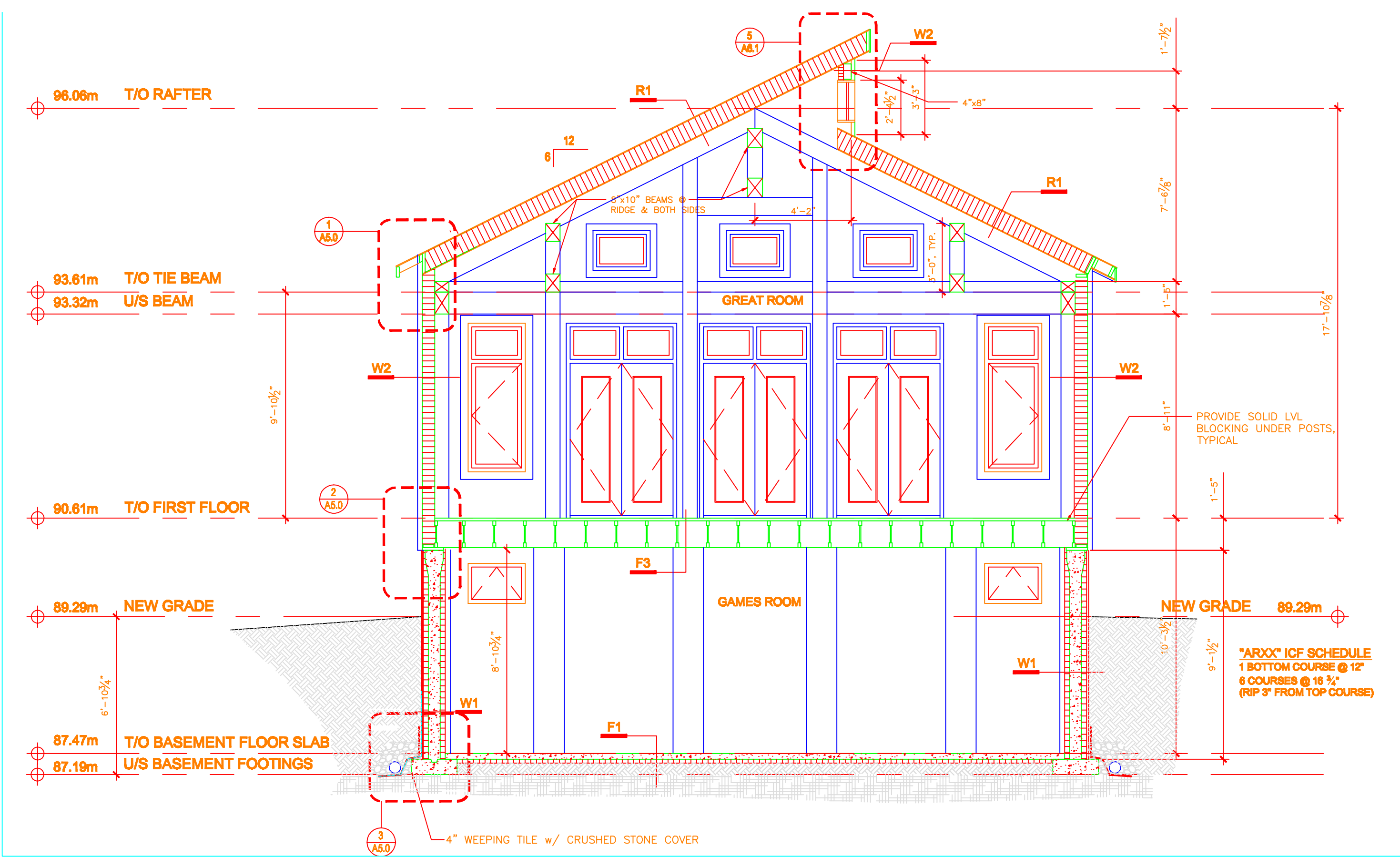
1 BUILDING SECTION SCALE: 1/4" = 1'
