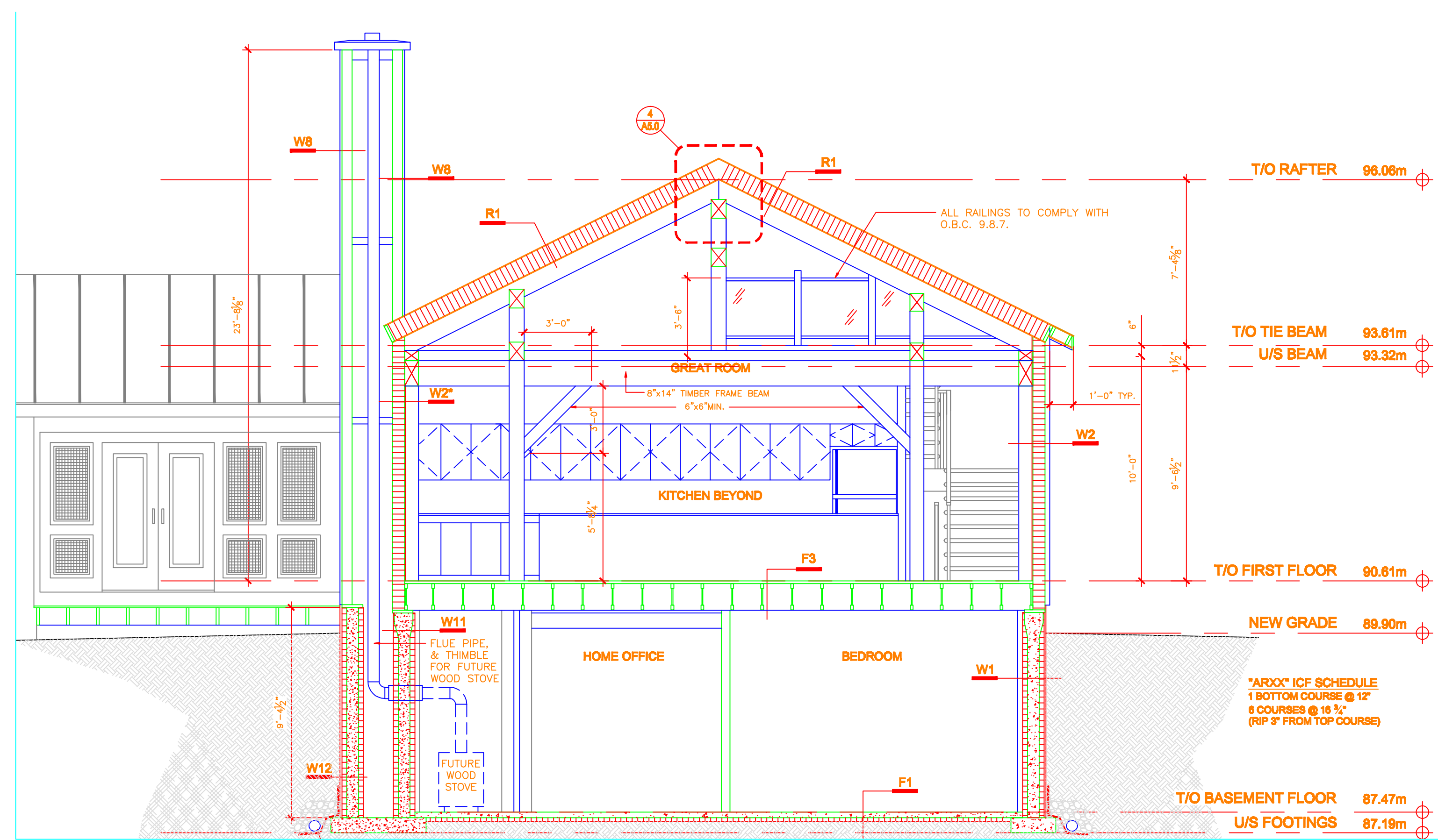
2 BUILDING SECTION SCALE: 1/4" = 1'
