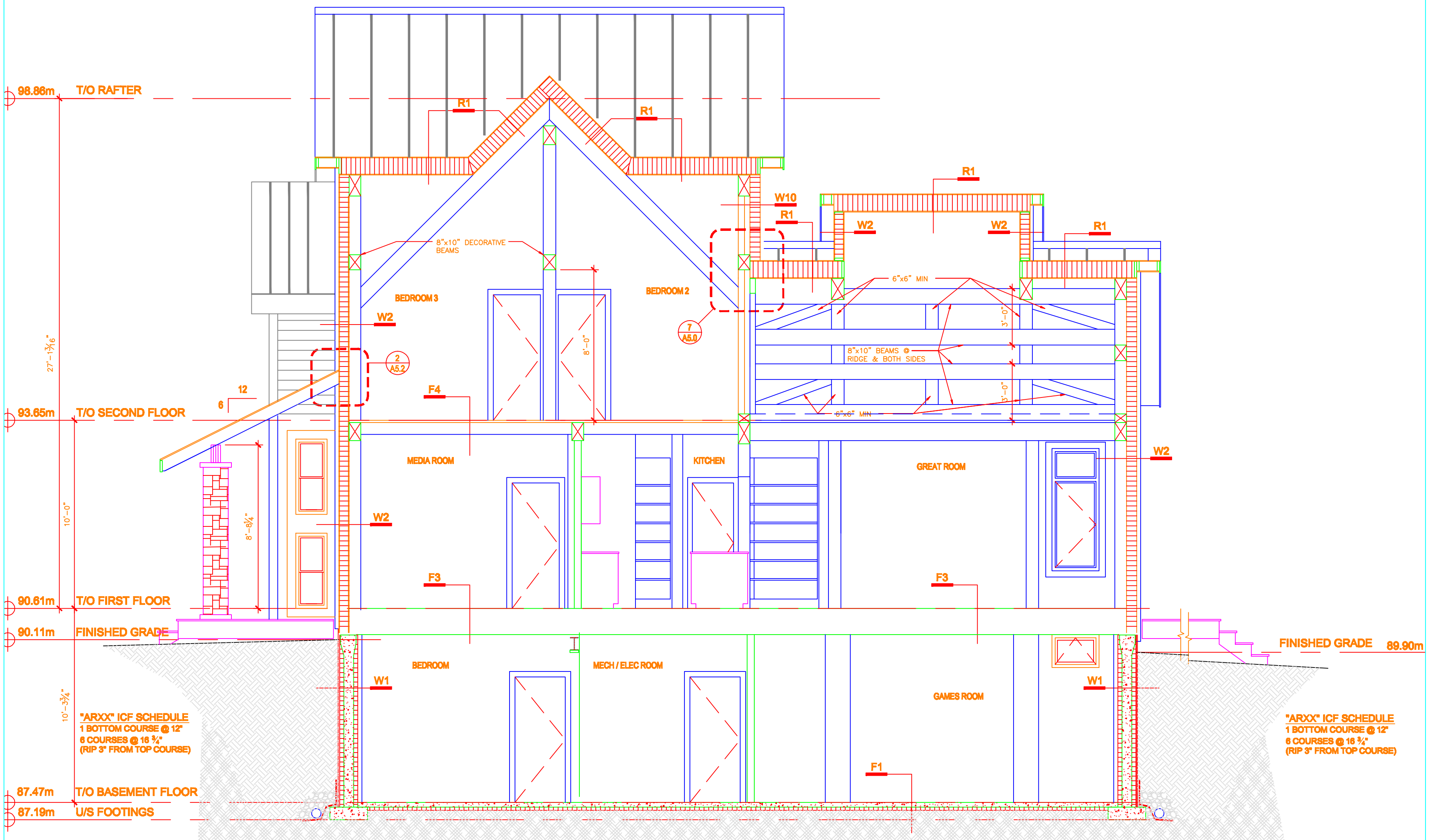
2 BUILDING SECTION SCALE: 1/4" = 1'
