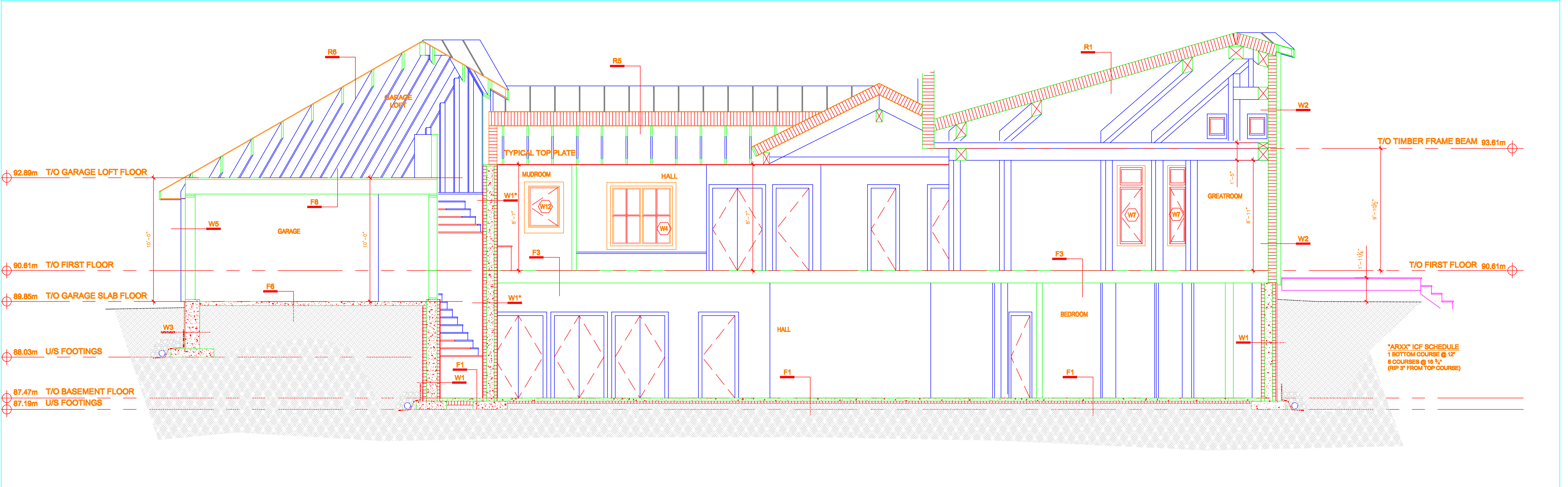
3 BUILDING SECTION SCALE: 1/4" = 1'
